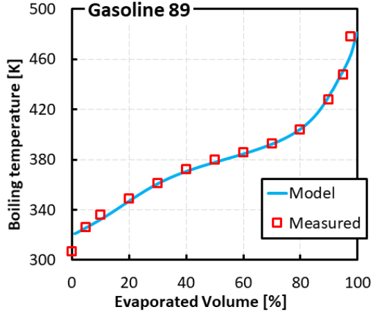
Figure 2-2: Comparison of distillation profile and fuel contents between the 13-component surrogate model in Table 2-2 and pump gasoline 89 fuel
