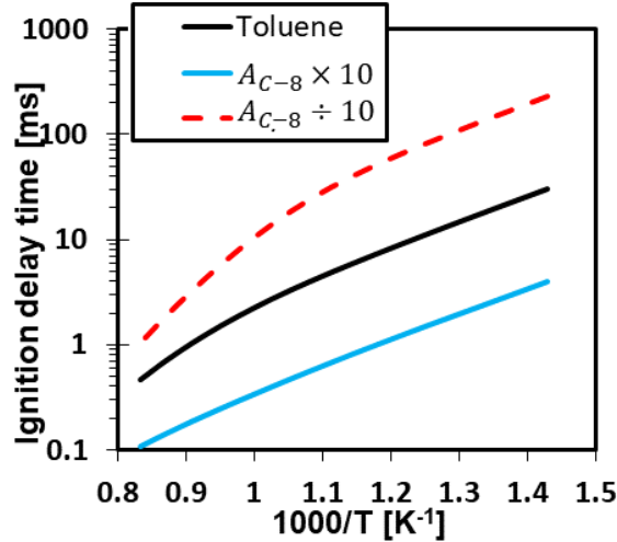
Figure 5-6: Sensitivity of IDT curve of toluene mechanism on reaction C-8, Benzyl + O_2 \leftrightarrow C_6H_5 + CH_2O + O
