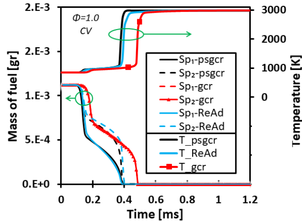
Figure 7-1: Mass and temperature variation of 2-component fuel ( Sp_1 is n-decane and Sp_2 is n-heptane). Simulated in a CV reactor with an initial pressure and temperature of 40 bar and 850K, respectively.
