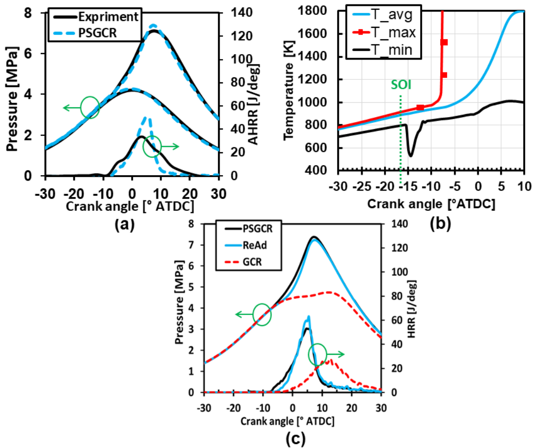
Figure 7-7: Comparison of (a) measured and predicted profiles of pressure and apparent heat release rate, (b) predicted maximum, minimum and average in-cylinder temperature based on the PSGCR model, (c) predicted pressure and heat release rate profiles based on different models
