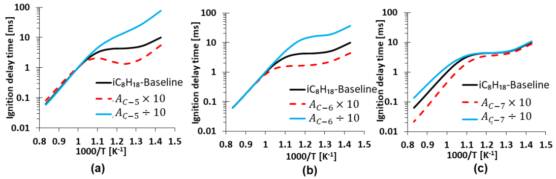
Figure 5-4: Sensitivity of IDT curve of iso-octane mechanism (a) reaction iC_8H_{18}+OH=iC_8H_{17}+H_2O , (b) reaction iC_8H_{17}O_2=iC_8H_{16}OOH , (c) reaction iC_8H_{18}+O_2=iC_8H_{17}+HO_2
